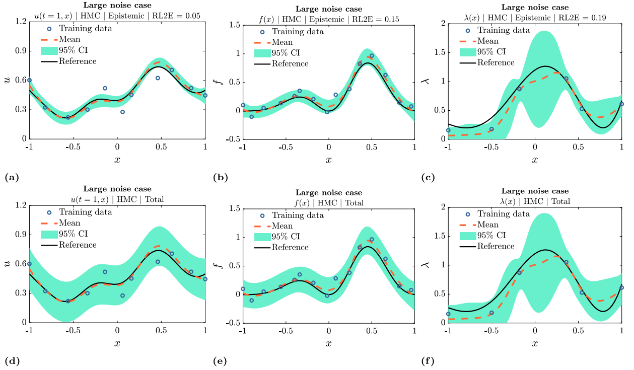
Fig. D.10. Mixed PDE problem of Eq. (21) – Large noise case: training data, reference functions, as well as mean and uncertainty (95% CI) predictions of HMC for u , f , and \lambda . Top row: epistemic uncertainty. Bottom row: total uncertainty including the known amount of aleatoric uncertainty, \sigma_u = 0.1 .
