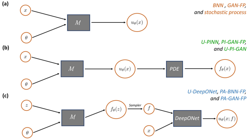
Fig. B.2. Repeated Fig. 8 from main text for convenience of the reader. (a) BNN, GAN functional prior (GAN-FP) and stochastic process representation. (b) U-PINN, PI-GAN-FP, and U-PI-GAN. (c) U-DeepONet, PA-BNN-FP, and PA-GAN-FP. \mathcal{M} expresses how x and \theta are combined to yield u_\theta(x) . In standard NN models (BNN, U-PINN, U-DeepONet), \mathcal{M} is a BNN. In generator-based models (stochastic process, FP, PI-GAN-FP, U-PI-GAN, and PA-GAN-FP), \mathcal{M} is the generator of a GAN that is trained using stochastic realizations or pre-trained using historical data. All models depicted in this figure can be construed as special cases of Fig. 10; note, however, the different meaning of \theta for each technique. Further, in part (c), \lambda (or both f and \lambda ) could be used as input to the DeepONet instead of f , as in Fig. 4. Furthermore, u(x; f) is equivalent to u(x; \xi) , because each \xi \in \Xi is associated with an input f . The additional input z is used to emphasize that the locations in the input domains of f and u can be different and the “sampler” that the function f_\theta(z) must be sampled at pre-specified locations before entered as input to the DeepONet. See Table 2 for an overview of the UQ methods and Table 15 for a glossary of used terms.
