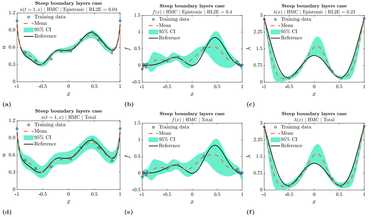
Fig. D.12. Mixed PDE problem of Eq. (21) — Steep boundary layers case: training data, reference functions, as well as mean and uncertainty (95% CI) predictions of HMC for u , f , and \lambda . Top row: epistemic uncertainty. Bottom row: total uncertainty including the known amount of aleatoric uncertainty, \sigma_u = 0.05 .
