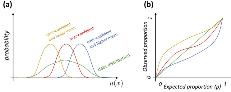
Fig. 12. Sketch of a data-generating distribution and indicative over-confident predictive models (a), and the corresponding calibration plots (b), for a given x . The calibration plot, for a given x , can be used to visualize the relationship between “expected proportion” of datapoints inside a statistical interval, which is p , and “observed proportion”, based on the predictive model, which is P(U_x \leq \hat{P}_x^{-1}(p)) . Note, however, that in practice for each x at most one sample u(x) is available, and thus the calibration plot is produced “on average” for different values of x . The observed proportions can be approximated via \mathbb{E}_{x,u \sim \mathcal{D}_{test}} \mathbb{1}\{u \leq \hat{u}(x)_p\} , where \hat{u}(x)_p is the inverse CDF value of the predictive model at x . An “ideal” predictive model matches the data distribution and its calibration plot is a straight line (green). An over-confident model (red) is typically above the green line for small values of p , and below the green line for larger values of p . The opposite is typically true for an under-confident model. Predictive models with different means compared to the data distribution (yellow, blue), may yield calibration plots that do not follow the aforementioned trends.
