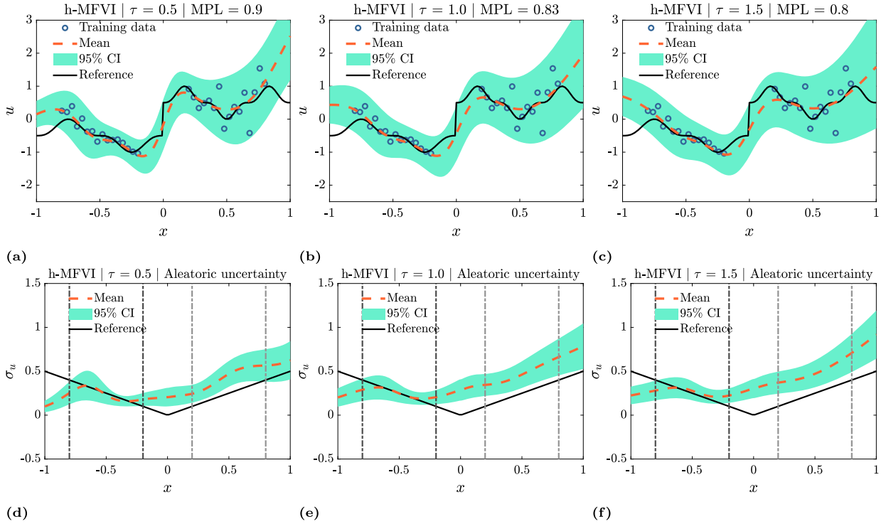
Fig. D.6. Function approximation problem of Eq. (20) — Unknown Student-t heteroscedastic noise : by modifying the “temperature” \tau we can control how conservative the predictions are. Here shown are h-MFVI predictions for three values of \tau (see Section A.4). Top row: mean and total uncertainty of u(x) . Bottom row: mean and epistemic uncertainty of predicted aleatoric uncertainty \sigma_u(x) . In the top row the training datapoints are also included, while in the bottom row the black and gray dot-dashed lines mark the training data intervals.
