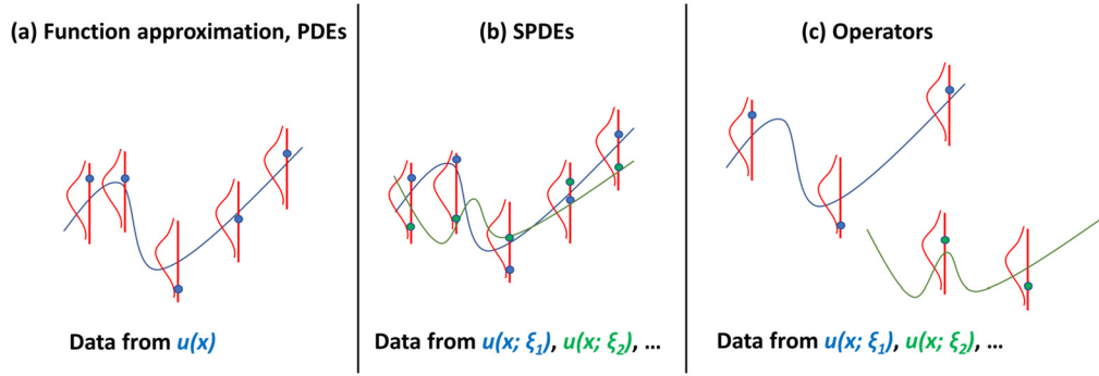
Fig. 13. Post-training calibration of uncertainty predictions: (a) for function approximation and deterministic PDE problems, calibration can be applied using data from u at different locations; (b) for solving SPDEs, using data from realizations (denoted with \xi ) of u at different locations; and (c) for neural operator learning, using data from u functions evaluated at different locations and corresponding to different \lambda inputs (or f , depending on which quantity is varying).
