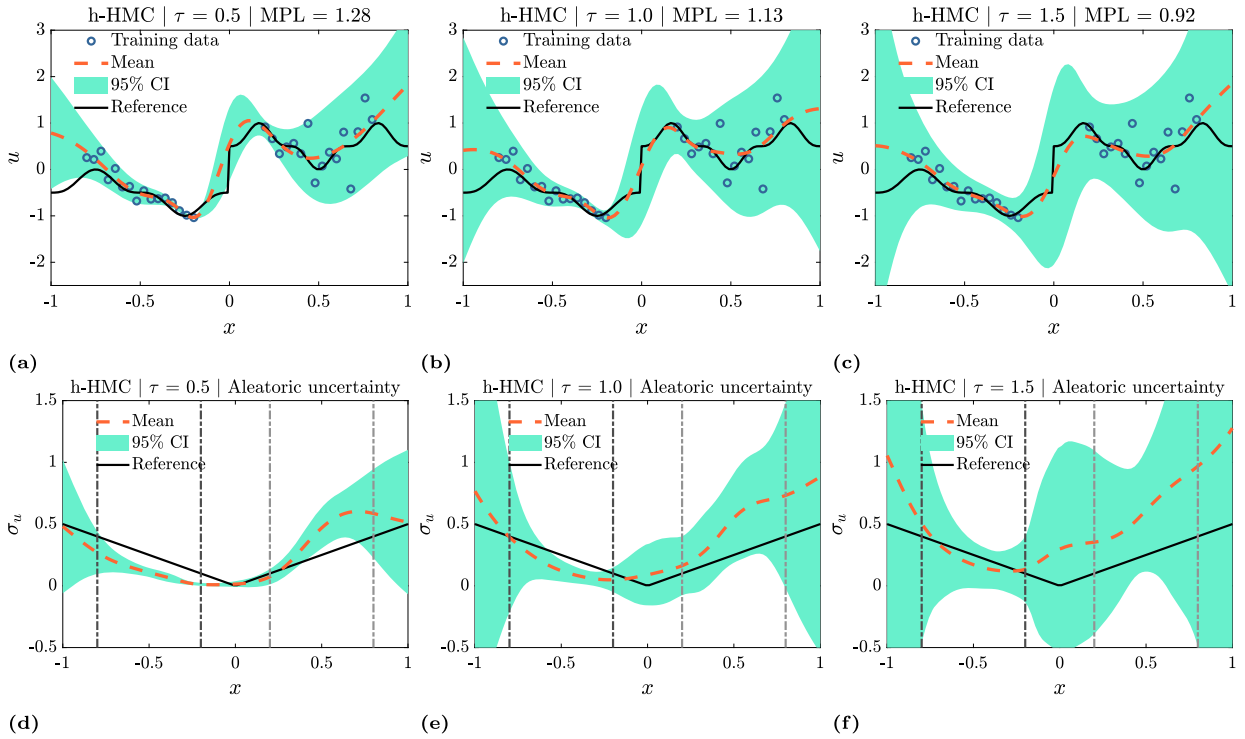
Fig. D.5. Function approximation problem of Eq. (20) — Unknown Student-t heteroscedastic noise : by modifying the “temperature” \tau we can control how conservative the predictions are. For this case of model misspecification, a cold posterior performs better in terms of predictive capacity (MPL); see also Table D.2. Note that data on the right side “happen” to be more noisy and this is reflected in the noise predictions. Here shown are h-HMC predictions for three values of \tau (see Section A.4). Top row: mean and total uncertainty of u(x) . Bottom row: mean and epistemic uncertainty of predicted aleatoric uncertainty \sigma_u(x) . In the top row the training datapoints are also included, while in the bottom row the black and gray dot-dashed lines mark the training data intervals.
