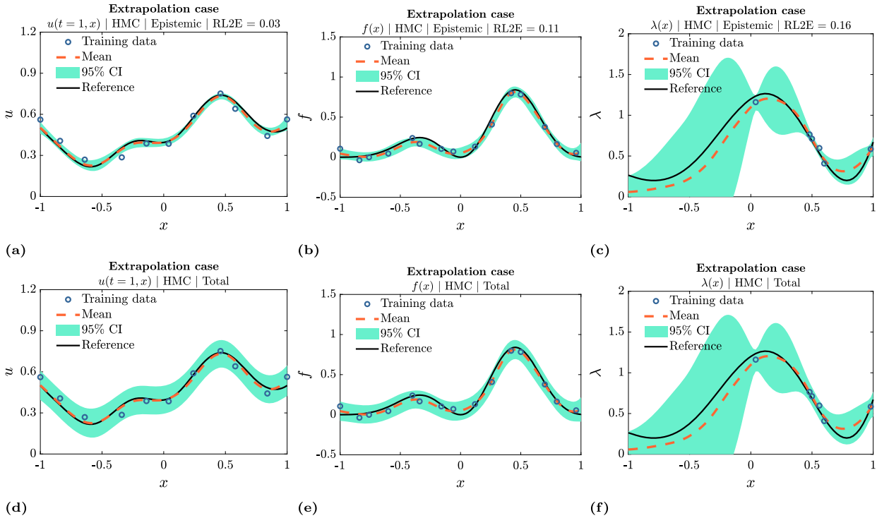
Fig. D.11. Mixed PDE problem of Eq. (21) – Extrapolation case: training data, reference functions, as well as mean and uncertainty (95% CI) predictions of HMC for u , f , and \lambda . Top row: epistemic uncertainty. Bottom row: total uncertainty including the known amount of aleatoric uncertainty, \sigma_u = 0.05 .
