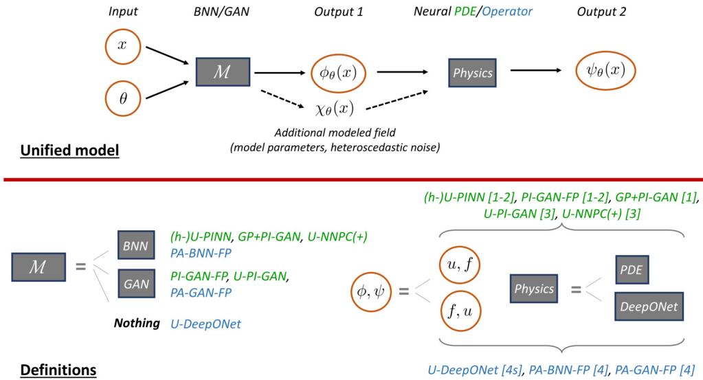
Fig. 10. A conceptual model towards a unified view of the presented techniques for addressing the problems of Fig. 1. We divide the methods into the ones that utilize a PDE describing the underlying physics ( neural PDEs ) and the ones that utilize a DeepONet as a surrogate model for the physics ( neural operators ). U-PINN and PI-GAN-FP address problems 1-2; GP+PI-GAN addresses problem 1; U-PI-GAN and U-NNPC(+) address problem 3; U-DeepONet, PA-BNN-FP, and PA-GAN-FP address problem 4. The model \mathcal{M} can be a BNN or the generator of a GAN, or nothing. The physics can be a PDE or a pre-trained DeepONet. The quantities \phi , \psi can be the solution u and the source f , or vice-versa; x represents the space-time input domain; and \theta represents the parameters of the BNN or the input noise to the GAN generator. Further, “ \chi ” can represent the model parameters \lambda in Eq. (1) and/or heteroscedastic noise. The numbers in the brackets correspond to the problems of Fig. 1, with “4s” referring to the special case of problem 4 (Section 1.2).
