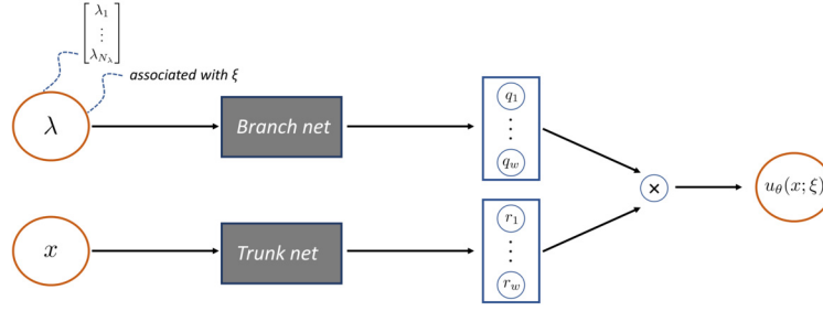
Fig. 4. The DeepONet architecture corresponding to output u_\theta(x; \xi) , where \xi is associated with an input function \lambda(x; \xi) . It consists of two sub-networks, one for the input x where the solution u is evaluated, called trunk net, and one for the input \lambda (a vector of size N_\lambda ), called branch net. The vectors [q_1, \dots, q_w] and [r_1, \dots, r_w] denote the outputs of the branch and trunk nets, respectively, and “ \times ” denotes their inner product. The model depicted in this figure can be construed as a special case of Fig. 10.
