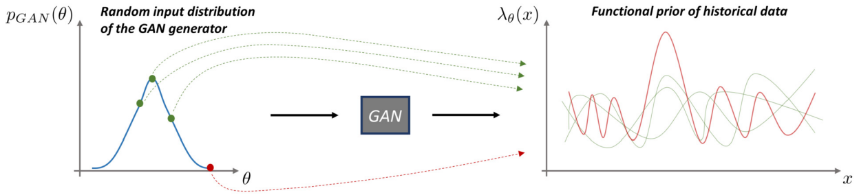
Fig. 35. The GAN-FP is trained such that drawing samples of \theta from p_{GAN}(\theta) produce \lambda functions that follow the historical data distribution. For OOD detection, we utilize the inverse of this relationship: a \lambda function that is far from the historical data distribution is expected to correspond to a \theta value that is far from the GAN input distribution. Values of \theta shown with green color on the left side are more probable under the distribution p_{GAN} and correspond to functions \lambda on the right side that have similar characteristics. On the other hand, the \theta value shown with red color is less probable and corresponds to a function \lambda that is different from the rest.
