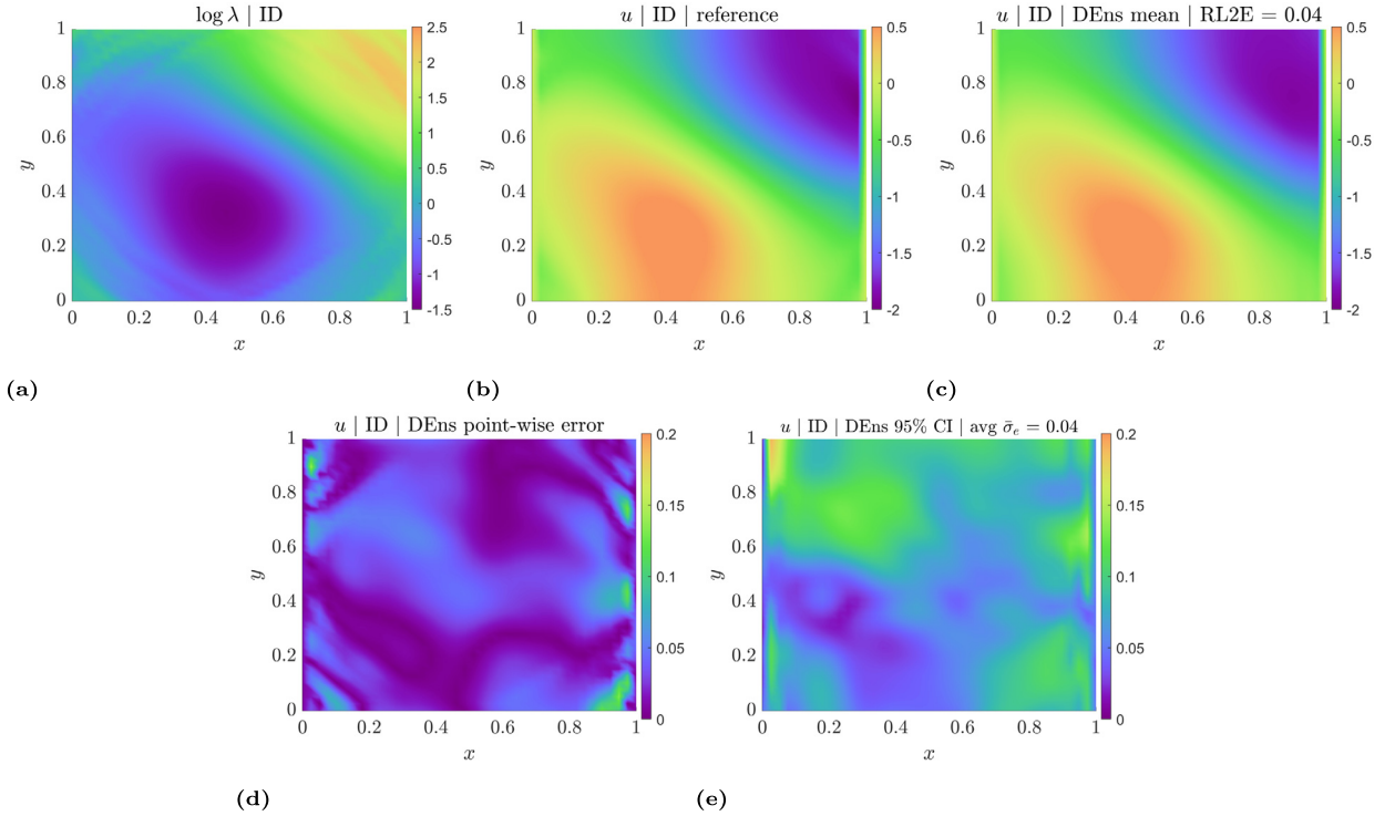
Fig. 32. Operator learning problem of Eqs. (29)–(30) — Complete and clean inference data of \lambda (ID data): the mean prediction of U-DeepONet, combined with DEns, approximates the solution u accurately with RL2E = 4%. Using each DeepONet separately, instead of a deep ensemble, would yield approximately the same error for ID data. Further, the 95% CI (approximately two standard deviations) of the epistemic uncertainty covers in all areas of the domain and follows spatially the absolute point-wise error of the mean. Here shown are the ID input \tilde{\lambda} = \log \lambda (a), the reference solution u (b), the mean of U-DeepONet (c), the absolute point-wise error of the mean (d), and the 95% CI of epistemic uncertainty (e).
