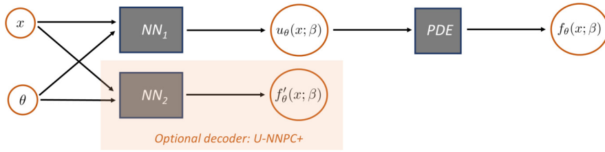
Fig. 9. NNPC, developed by [138], and NNPC+ (orange box), proposed herein, for solving SPDEs. NNs 1 and 2, parametrized by \beta , combine the location in the domain x to produce the modes of the stochastic representations of u_\theta(x; \beta) and f'_\theta(x; \beta) , respectively. The model depicted in this figure can be construed as a special case of Fig. 10; note, however, the different meaning of \theta in this technique.
