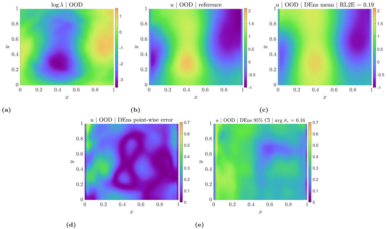
Fig. 33. Operator learning problem of Eqs. (29)–(30) — Complete and clean inference data of \lambda (OOD data): although the mean prediction of U-DeepONet, combined with DEns, has RL2E = 19%, the value of the same metric would be 40% if a deep ensemble were not used. This fact demonstrates the potency of U-DeepONet, as compared to standard DeepONet, for treating OOD data. Further, the 95% CI (approximately two standard deviations) of the epistemic uncertainty covers the absolute error of the mean in all areas of the domain. Here shown are the OOD input \lambda = \log \lambda (a), the reference solution u (b), the mean of U-DeepONet (c), the absolute point-wise error of the mean (d), and the 95% CI of epistemic uncertainty (e).
