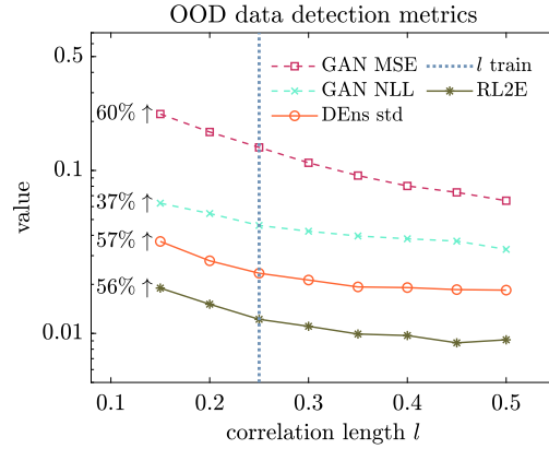
Fig. 34. Operator learning problem of Eqs. (29)–(30) — OOD data detection: the three proposed OOD data detection metrics of Table 13, namely, GAN MSE, GAN NLL, and DEns std, follow the RL2E trend. Here shown are the metric values for inputs \lambda associated with a truncated GP of the form of Eq. (31) with different correlation lengths. The RL2E of U-DeepONet as well as the correlation length used in the U-DeepONet pre-training phase are also included for comparisons. All values are averaged over 100 \lambda inputs.
