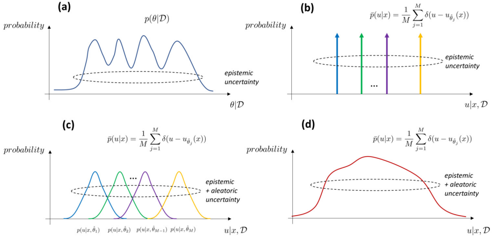
Fig. 5. Total uncertainty represented by the predictive distribution \bar{p}(u|x) : (a) Epistemic uncertainty is taken into account via the posterior p(\theta|\mathcal{D}) , (b) p(\theta|\mathcal{D}) is approximated via representative samples \{\hat{\theta}_j\}_{j=1}^M , (c) aleatoric uncertainty is added to each sample from p(\theta|\mathcal{D}) via the distributions \{p(u|x, \hat{\theta}_j)\}_{j=1}^M , (d) \bar{p}(u|x) approximates total uncertainty by adding up the distributions \{p(u|x, \hat{\theta}_j)\}_{j=1}^M . If each p(u|x, \hat{\theta}_j) is a Gaussian distribution, \bar{p}(u|x) corresponds to a Gaussian mixture. See Table 15 for a glossary of used terms.
