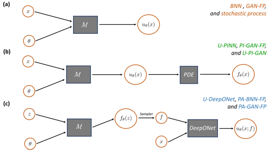
Fig. 8. (a) BNN, GAN functional prior (GAN-FP) and stochastic process representation. (b) U-PINN, PI-GAN-FP, and U-PI-GAN. (c) U-DeepONet, PA-BNN-FP, and PA-GAN-FP. \mathcal{M} expresses how x and \theta are combined to yield u_\theta(x) . In standard NN models (BNN, U-PINN, U-DeepONet), \mathcal{M} is a BNN. In generator-based models (stochastic process, FP, PI-GAN-FP, U-PI-GAN, and PA-GAN-FP), \mathcal{M} is the generator of a GAN that is trained using stochastic realizations or pre-trained using historical data. All models depicted in this figure can be construed as special cases of Fig. 10; note, however, the different meaning of \theta for each technique. Further, in part (c), \lambda (or both f and \lambda ) could be used as input to the DeepONet instead of f , as in Fig. 4. Furthermore, u(x; \xi) is equivalent to u(x; \xi) , because each \xi \in \Xi is associated with an input f . The additional input z is used to emphasize that the locations in the input domains of f and u can be different and the “sampler” that the function f_\theta(z) must be sampled at pre-specified locations before entered as input to the DeepONet. See Table 2 for an overview of the UQ methods and Table 15 for a glossary of used terms.
