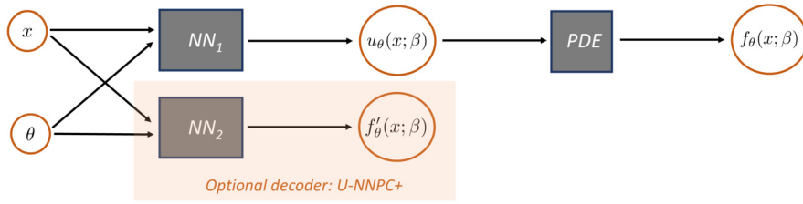
Fig. B.3. Repeated Fig. 9 from main text for convenience of the reader. NNPC, developed by [138], and NNPC+ (orange box), proposed herein, for solving SPDEs. NNs 1 and 2, parametrized by \beta , combine the location in the domain x to produce the modes of the stochastic representations of u_\theta(x; \beta) and f'_\theta(x; \beta) , respectively. The model depicted in this figure can be construed as a special case of Fig. 10; note however the different meaning of \theta in this technique.
