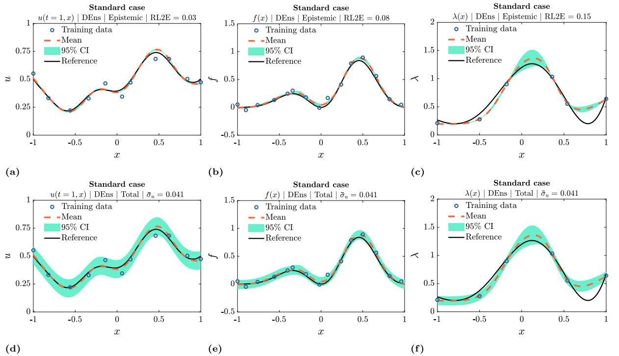
Fig. 24. Mixed PDE problem of Eq. (21) – Standard case : DEns estimates \lambda(x) more accurately than HMC, although it is over-confident (small epistemic uncertainty). Shown here are the training data, reference functions, as well as the mean and uncertainty (95% CI) predictions of DEns for u , f , and \lambda . Top row : epistemic uncertainty. Bottom row : total uncertainty including the learned amount of aleatoric uncertainty, \bar{\sigma}_u = 0.041 .
