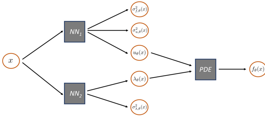
Fig. 7. PINN consisting of two NNs, one for the solution u and one for the parameter field \lambda . The parameters of the NNs are denoted by \theta . We also consider heteroscedastic Gaussian noise in the data of f , u , and \lambda , whose variances are denoted by \sigma^2_{f,\theta} , \sigma^2_{u,\theta} , and \sigma^2_{\lambda,\theta} , respectively. We refer to this model as h-U-PINN in Table 2; i.e., PINN with heteroscedastic noise modeling and parameters \theta obtained through posterior inference. Related computational results can be found in Section 6.2.2. The model depicted in this figure can be construed as a special case of Fig. 10 with additional NN outputs for the noise variances.
