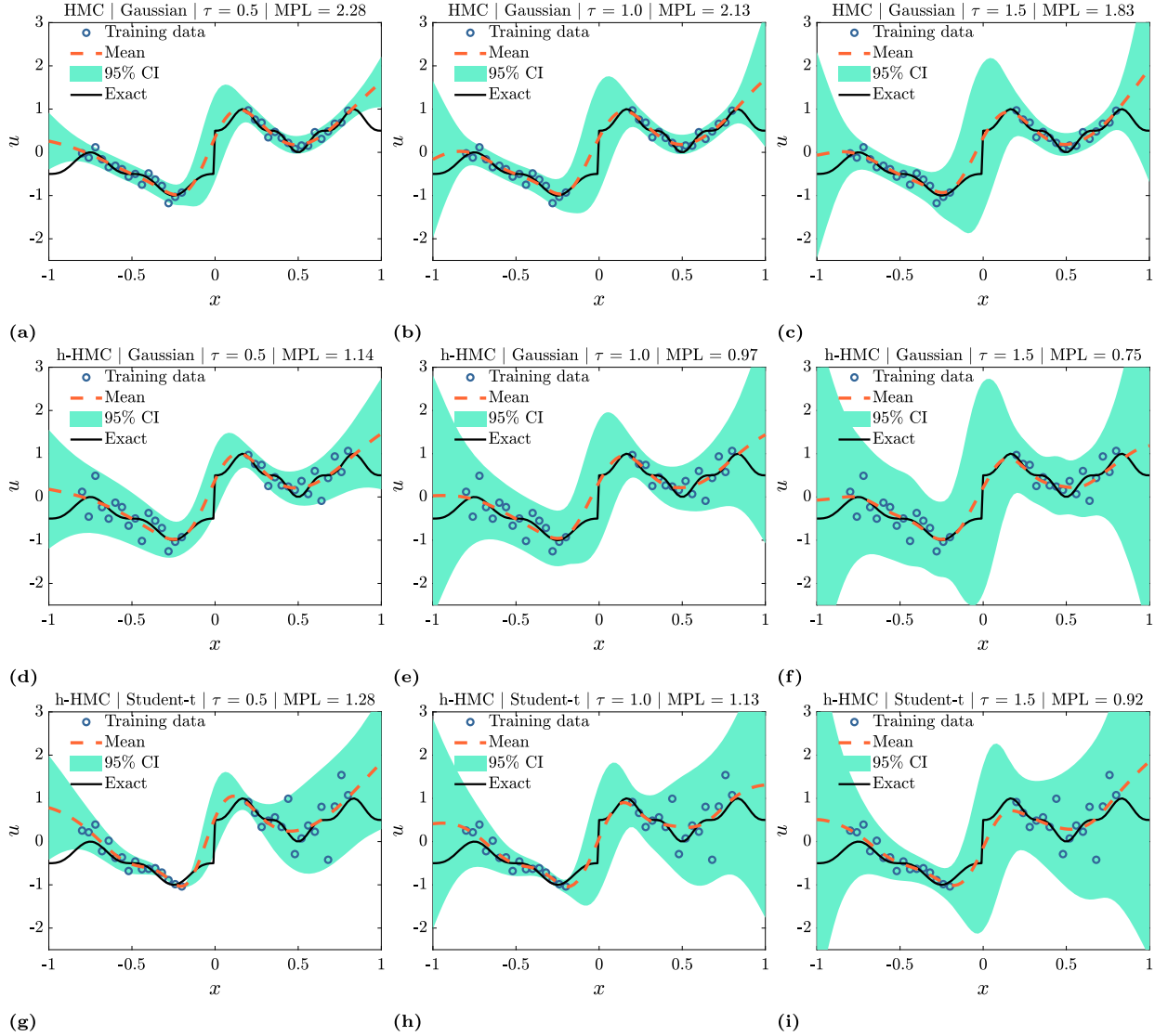
Fig. D.7. Function approximation problem of Eq. (20) – Gaussian or Student-t noise: posterior tempering (Section A.4) can be construed as including one additional hyperparameter in the training procedure. Thus, it can be used both for cases where the assumed model is correct (a-c) and for model misspecification cases (d-i). Here shown are the mean and total uncertainty predictions of uncalibrated HMC for different posterior temperatures. Top row: known homoscedastic Gaussian noise. Middle row: unknown heteroscedastic Gaussian noise. Bottom row: unknown heteroscedastic Student-t noise.
